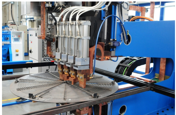
IDEAL cnc jig welder with fan grid
